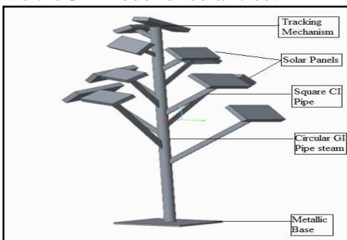
Figure. 2 3D model of solar tree
