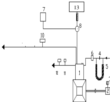
Figure-2. Schematic Diagram of Experimental Set-up
