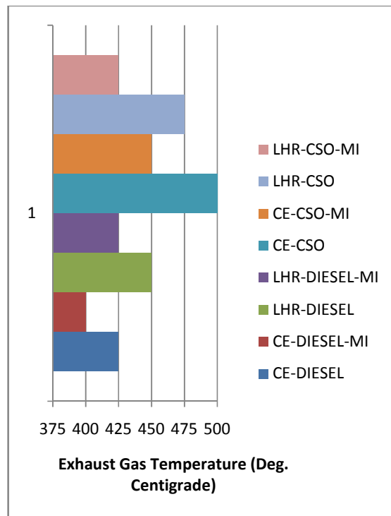
Figure-8 Bar chart showing the variation of exhaust gas temperature at full load with different versions of the engine with test fuels with and without magnetic induction.
