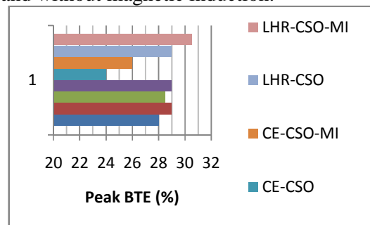
Figure - 6 Bar chart showing the variation of peak brake thermal efficiency (BTE) with different versions of the engine with test fuels with and without magnetic induction
