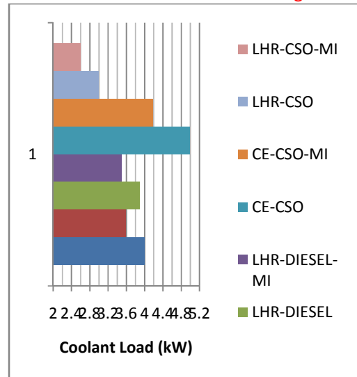
Figure-9 Bar chart showing the variation of coolant load at full load with different versions of the engine with test fuels with and without magnetic induction
