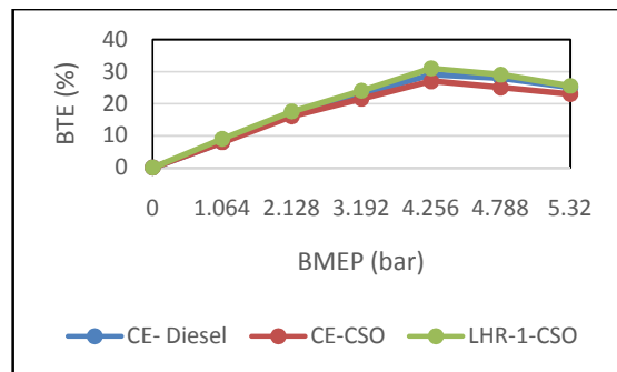
Figure- 5 Variation of brake thermal efficiency (BTE) with brake mean effective pressure(BMEP) of the engine with magnetic induction
