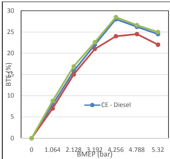
Figure- 4 Variation of brake thermal efficiency (BTE) with brake mean effective pressure (BMEP) of the engine without magnetic induction
