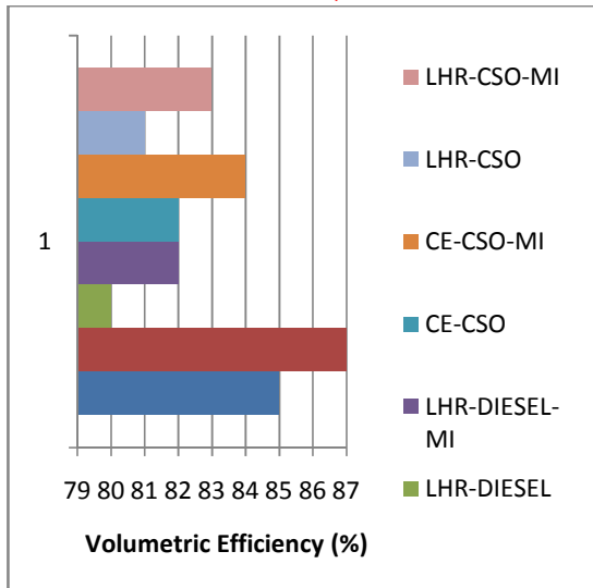
Figure-10 Bar chart showing the variation of volumetric efficiency at full load with different versions of the engine with test fuels with and without magnetic induction
