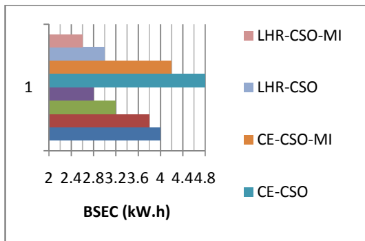
Figure-7 Bar chart showing the variation of brake specific energy consumption (BSEC) at full load with different versions of the engine with test fuels with and without magnetic induction
