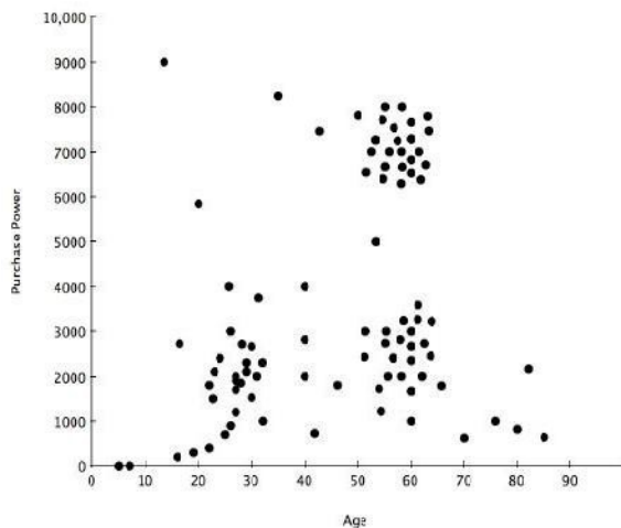
Figure - 1 Clustering
