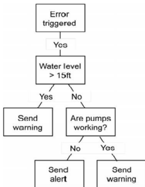
Figure 2. Decision tree
