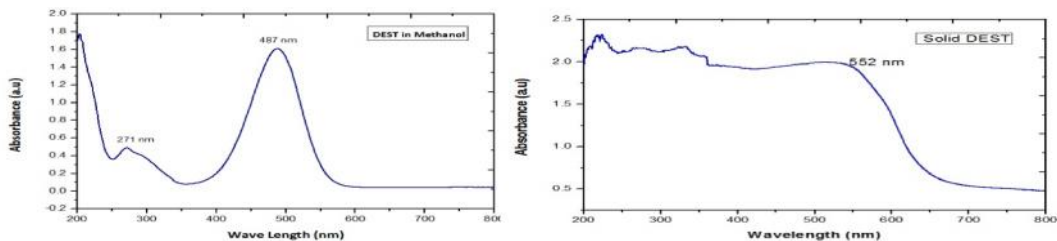
Figure 2- Absorption spectrum of DESI single crystal
