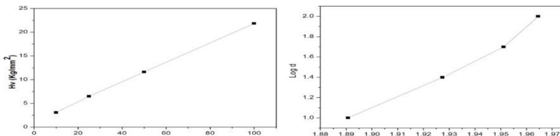
Figure 3a -Variation of H_v (Vickers hardness) with load ( P ) and 3b. Graph between \log p vs \log d
