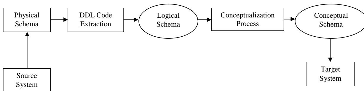
Figure.2.2. A framework for Database Reverse Engineering (DBRE)
